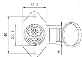
推荐面板安装尺寸 Recommended Panel Mounting Dimensions
