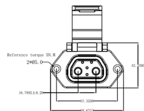
推荐面板安装尺寸 Recommended Panel Mounting Dimensions
