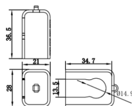
推荐面板安装尺寸 Recommended Panel Mounting Dimensions
