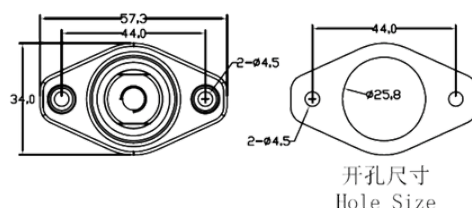
推荐面板安装尺寸 Recommended Panel Mounting Dimensions
