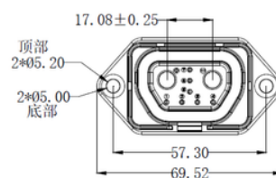
推荐面板安装尺寸 Recommended Panel Mounting Dimensions
