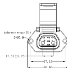
推荐面板安装尺寸 Recommended Panel Mounting Dimensions
