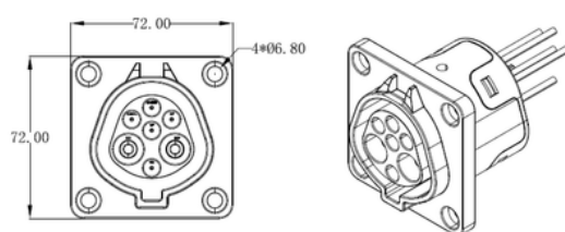
推荐面板安装尺寸 Recommended Panel Mounting Dimensions
