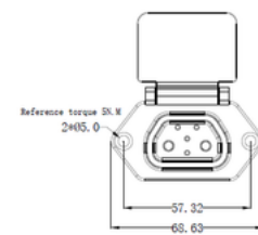
推荐面板安装尺寸 Recommended Panel Mounting Dimensions
