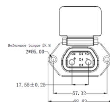
推荐面板安装尺寸 Recommended Panel Mounting Dimensions
